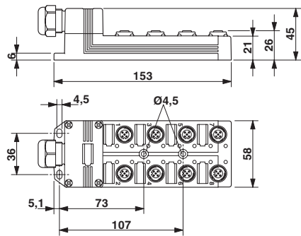
Dimensional drawing
