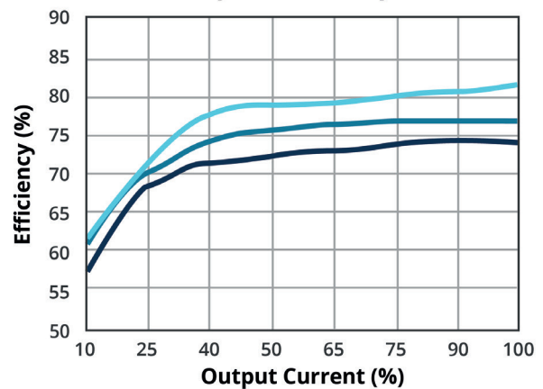
EFFICIENCY VS OUTPUT LOAD (Vin = 230 VAC)
